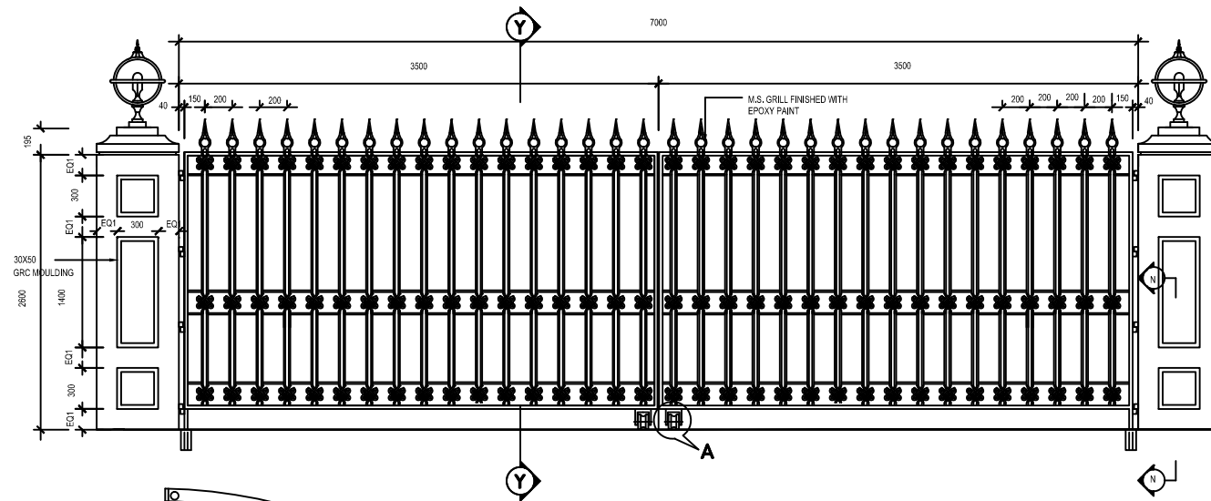
ELEVATION OF M.S. GATE 1:20
