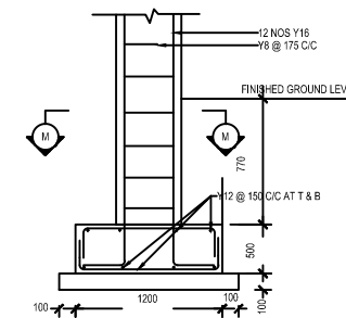
SECTION N-N
