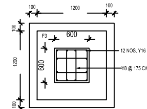
SECTION M-M
