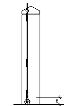
SECTION Y-Y 1:20
