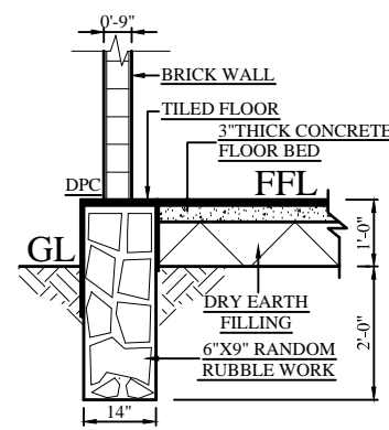
DETAIL OF WALL FOUNDATION
