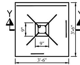
PLAN DETAIL OF R.C.C. COLUMN
