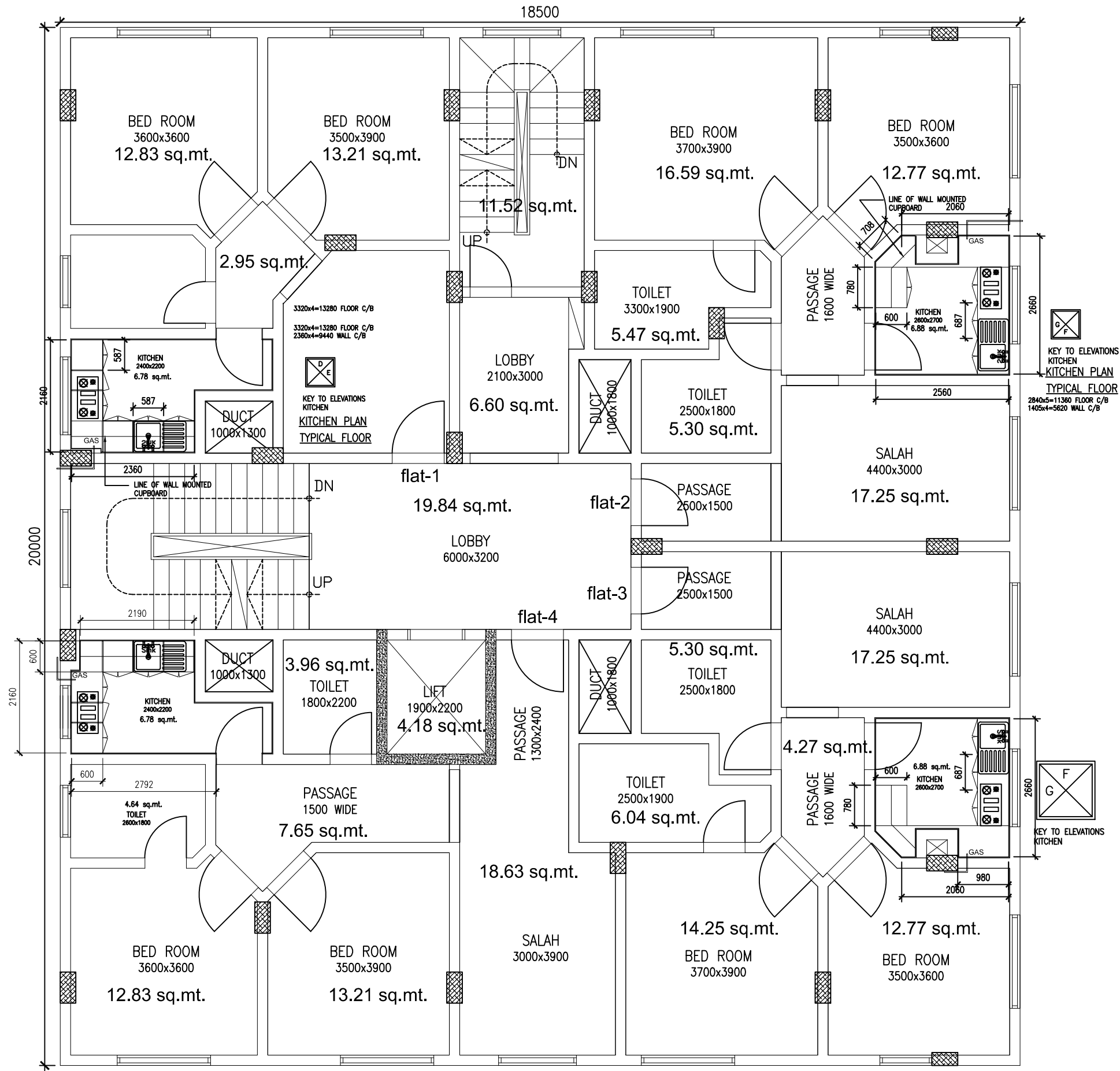
TYPICAL 1,2,3&4 FLOOR PLAN
